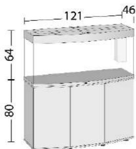
Maße: 121x46x64/80cm | ca. 260L 2x 29W LED (1047mm) | Bioflow L Eccoflow 1000 | AquaHeat Pro 300W
