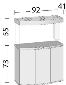
Maße: 92x41x55/73cm | ca. 180L 2x 19W LED (742mm) | Bioflow M Eccoflow 600 | AquaHeat Pro 200W
