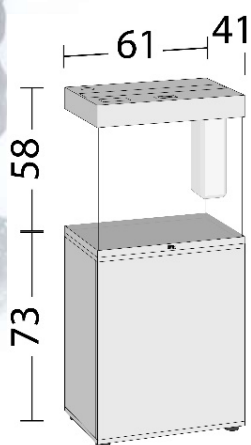
Maße: 61x41x58/73cm | ca. 120L 2x 12W LED (438mm) | Bioflow M Eccoflow 500 | AquaHeat Pro 100W
